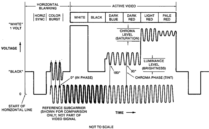
Fig. 8-2. Video waveform for one horizontal scan line.
